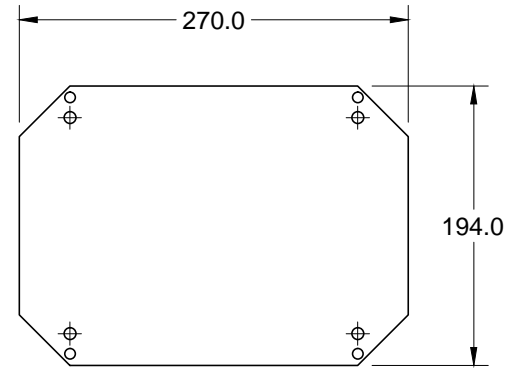
MOUNTING PLATE
