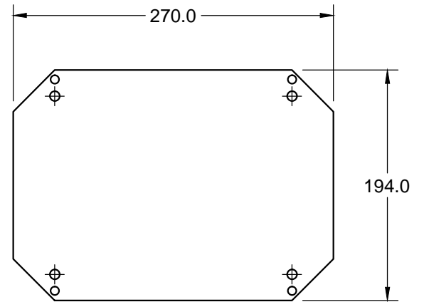
MOUNTING PLATE
