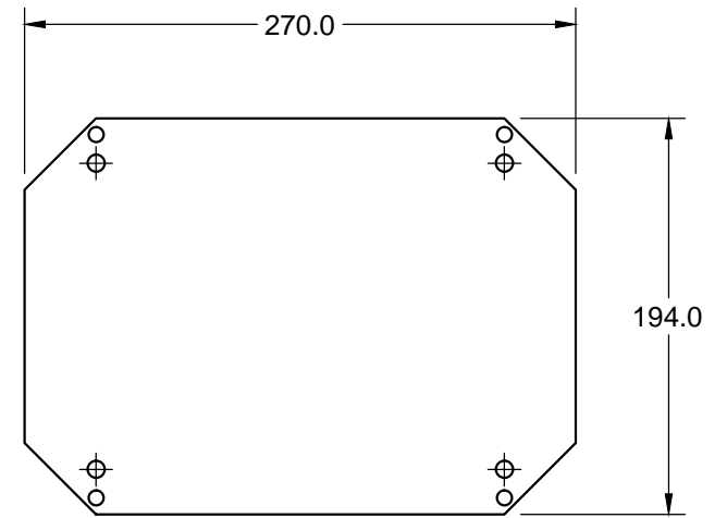
MOUNTING PLATE
