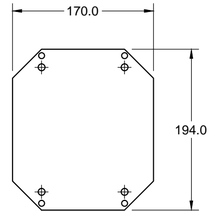
MOUNTING PLATE
