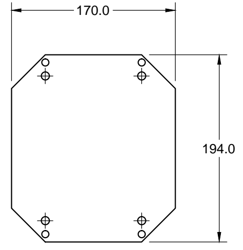
MOUNTING PLATE
