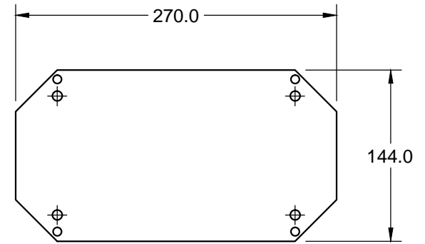
MOUNTING PLATE
