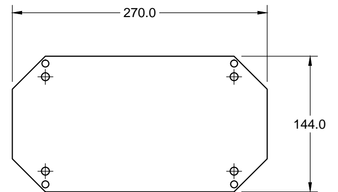
MOUNTING PLATE
