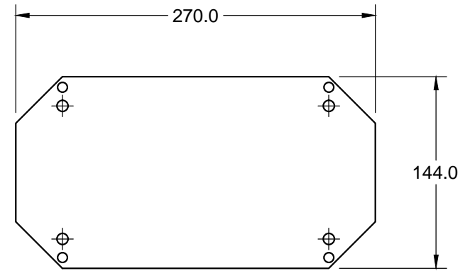
MOUNTING PLATE
