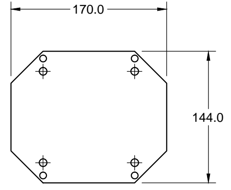
MOUNTING PLATE
