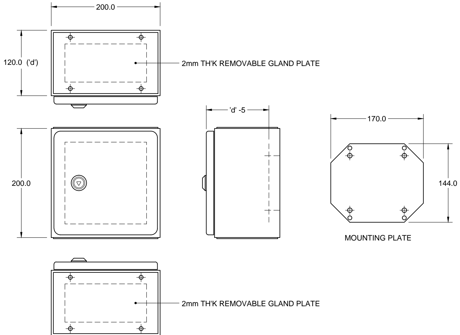
'CF' ENCLOSURE 200 HIGH 200 WIDE 120 DEEP
